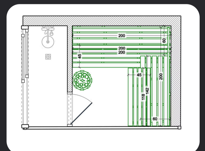
Layout of wooden furniture and the Shower system
