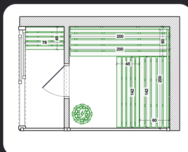
Layout of wooden furniture and the stove
