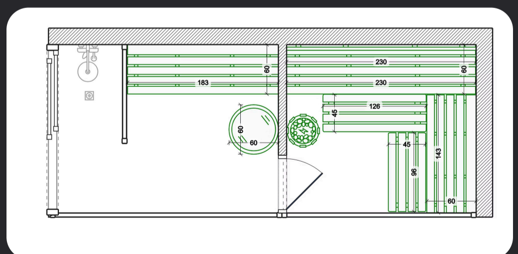
Layout of wooden furniture and the stove
